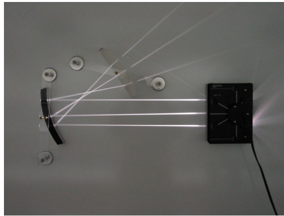
Ray Tracing
